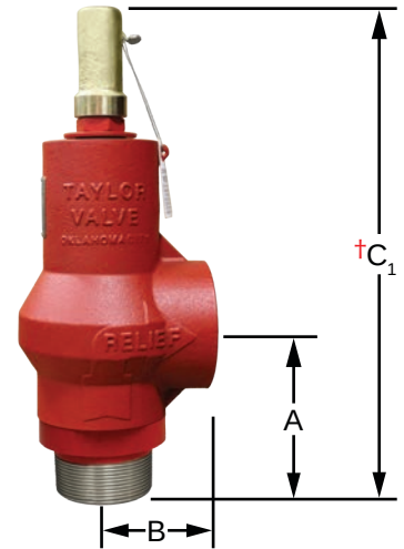
3" THREADED VALVE
