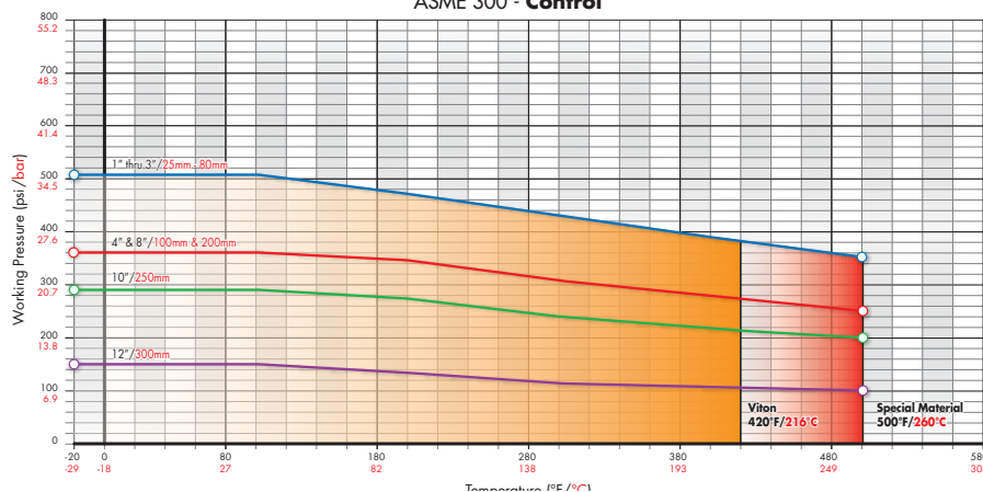
ASME 300 - Shut-Off
