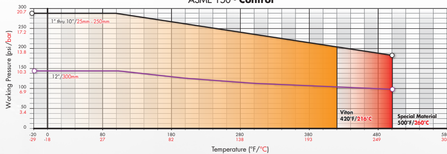
ASME 150 - Control
